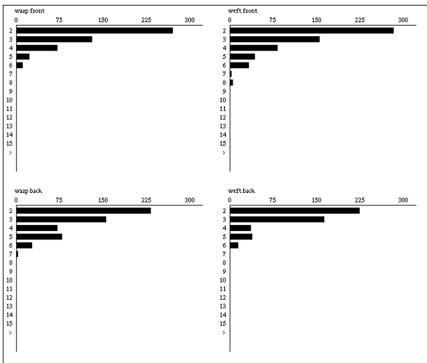
Figure 6. Weft-Choice Floats
