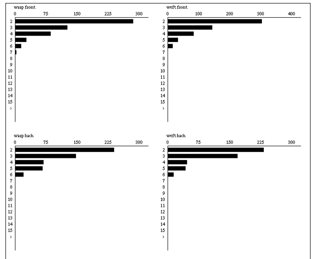
Figure 7. Alternating-Choice Floats
