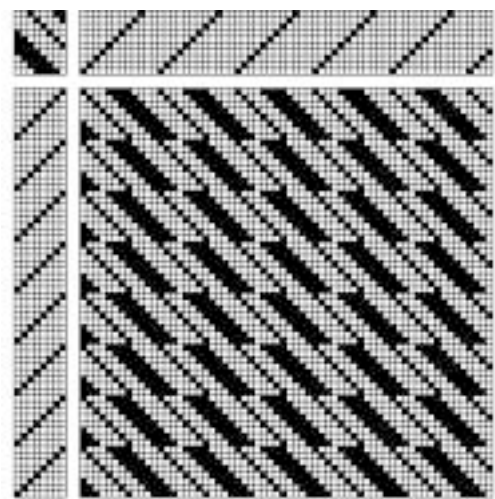
Figure 11. ↗ ↗ Draws with 8×12 /1/4/3 Twill
