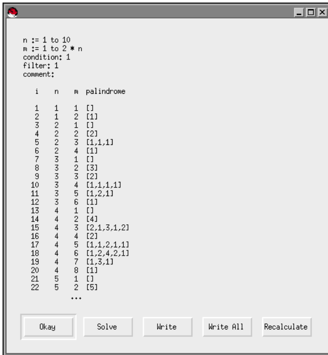
Figure 2. Result Dialog
