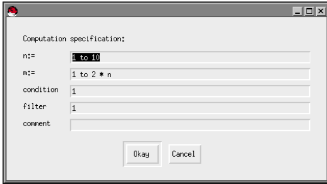
Figure 1. Specification Dialog
