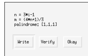
Figure 5. Formulas for 1, 1, 1
