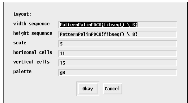
Figure 6. A Fibonacci Layout
